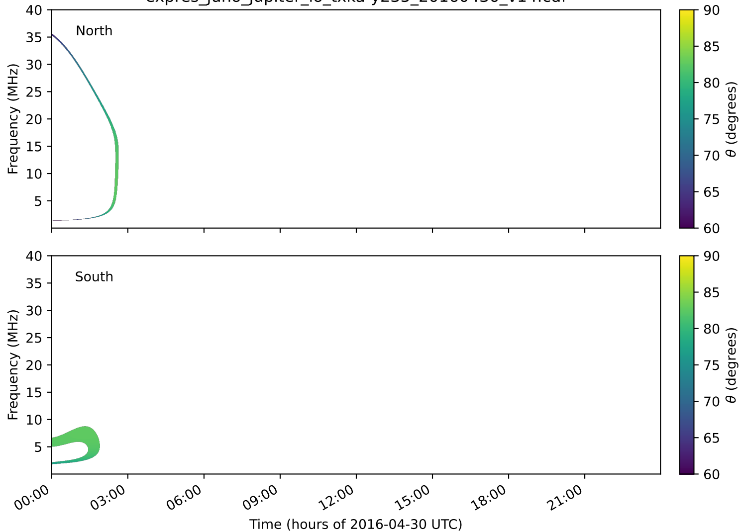
expres_juno_jupiter_io_txka-y235_20160430_v14.cdf
