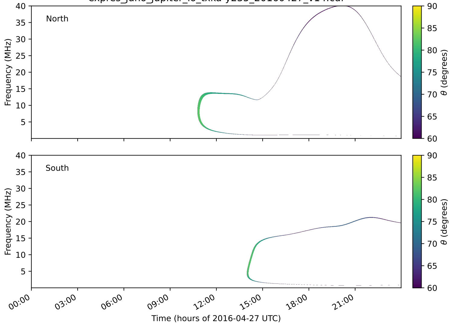
expres_juno_jupiter_io_txka-y235_20160427_v14.cdf
