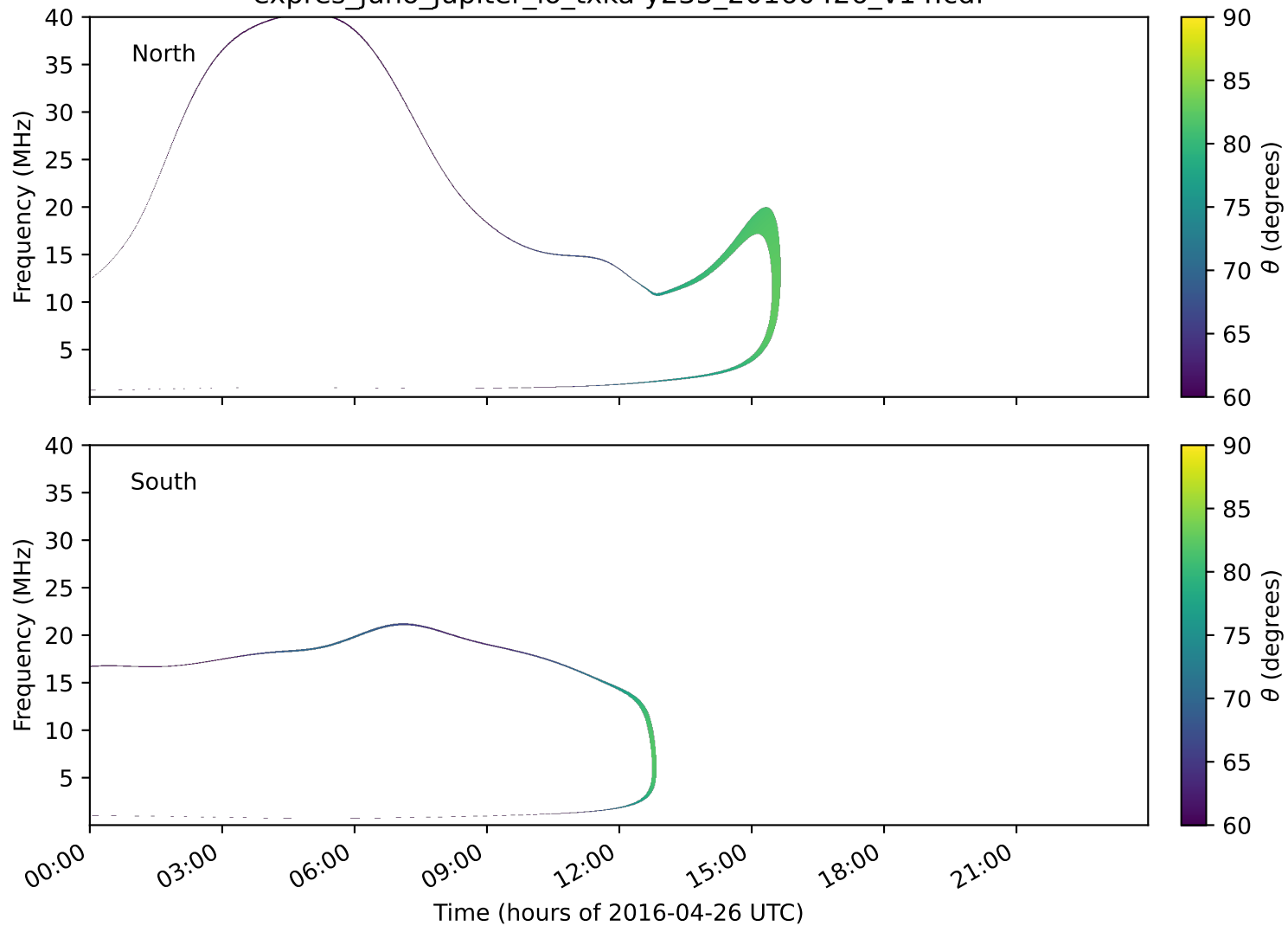
expres_juno_jupiter_io_txka-y235_20160426_v14.cdf
