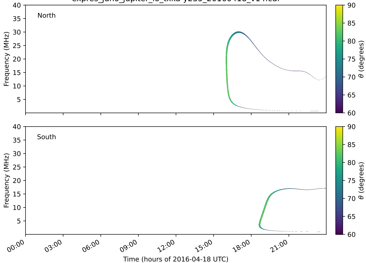
expres_juno_jupiter_io_txka-y235_20160418_v14.cdf
