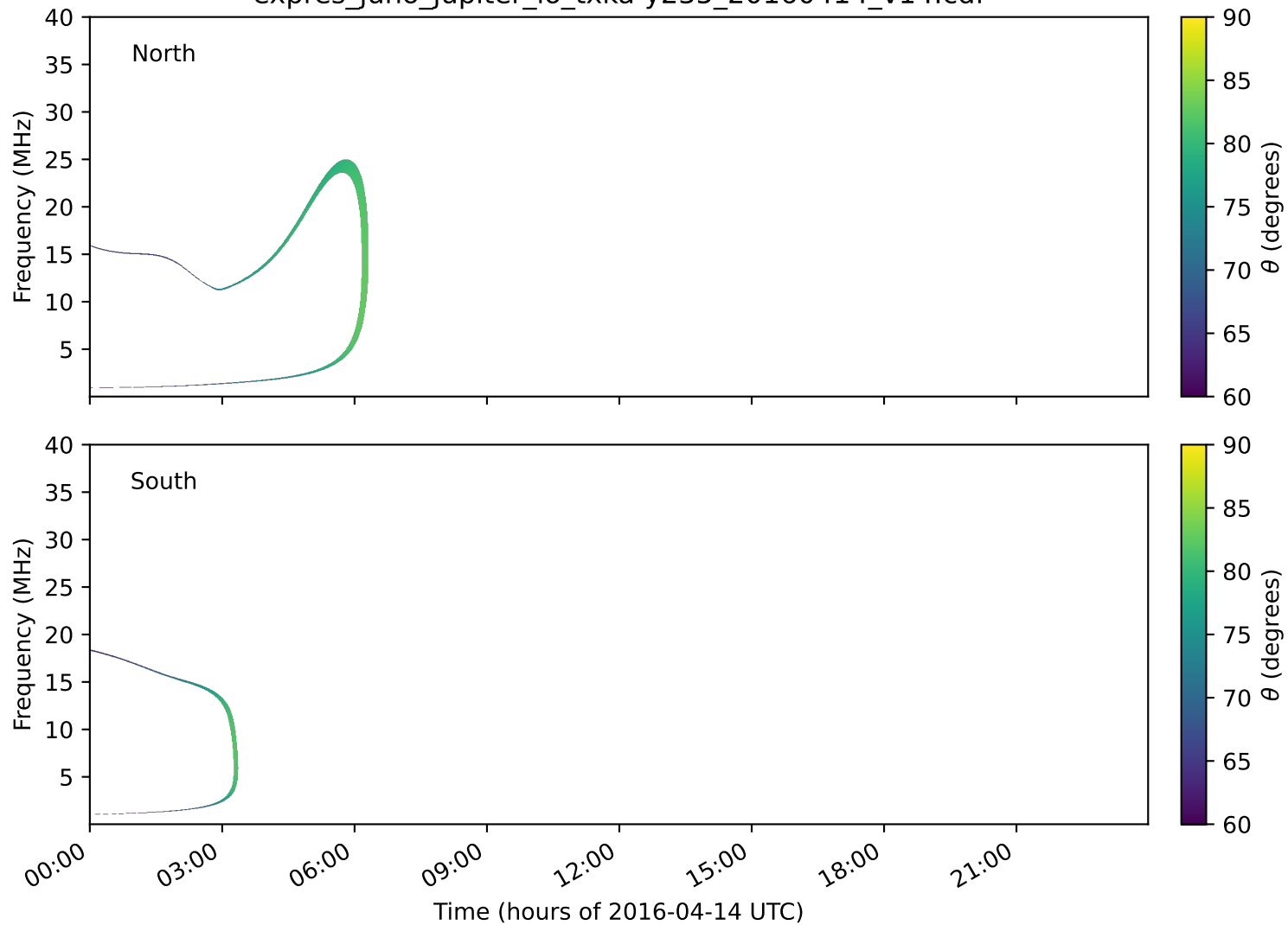
expres_juno_jupiter_io_txka-y235_20160414_v14.cdf
