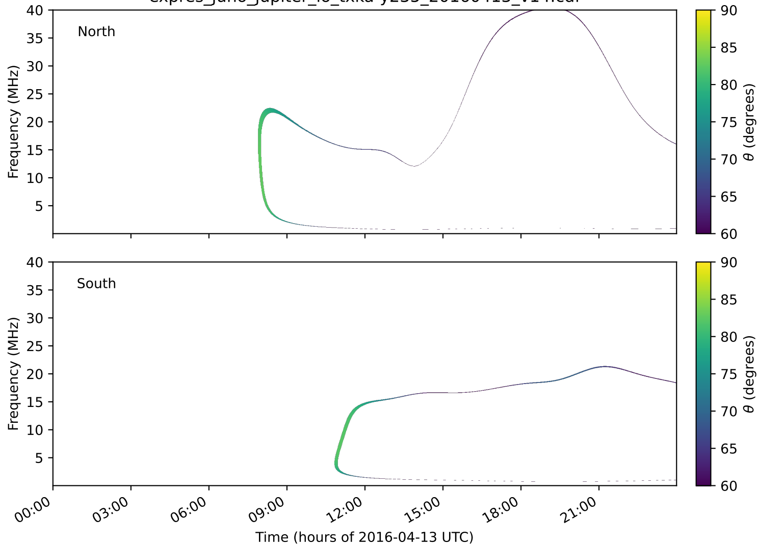
expres_juno_jupiter_io_txka-y235_20160413_v14.cdf
