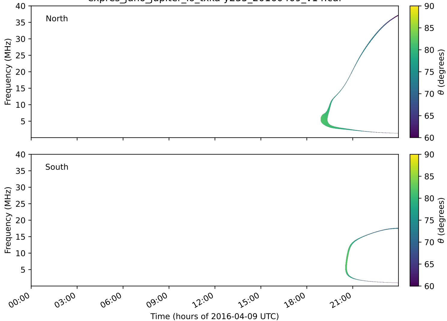
expres_juno_jupiter_io_txka-y235_20160409_v14.cdf
