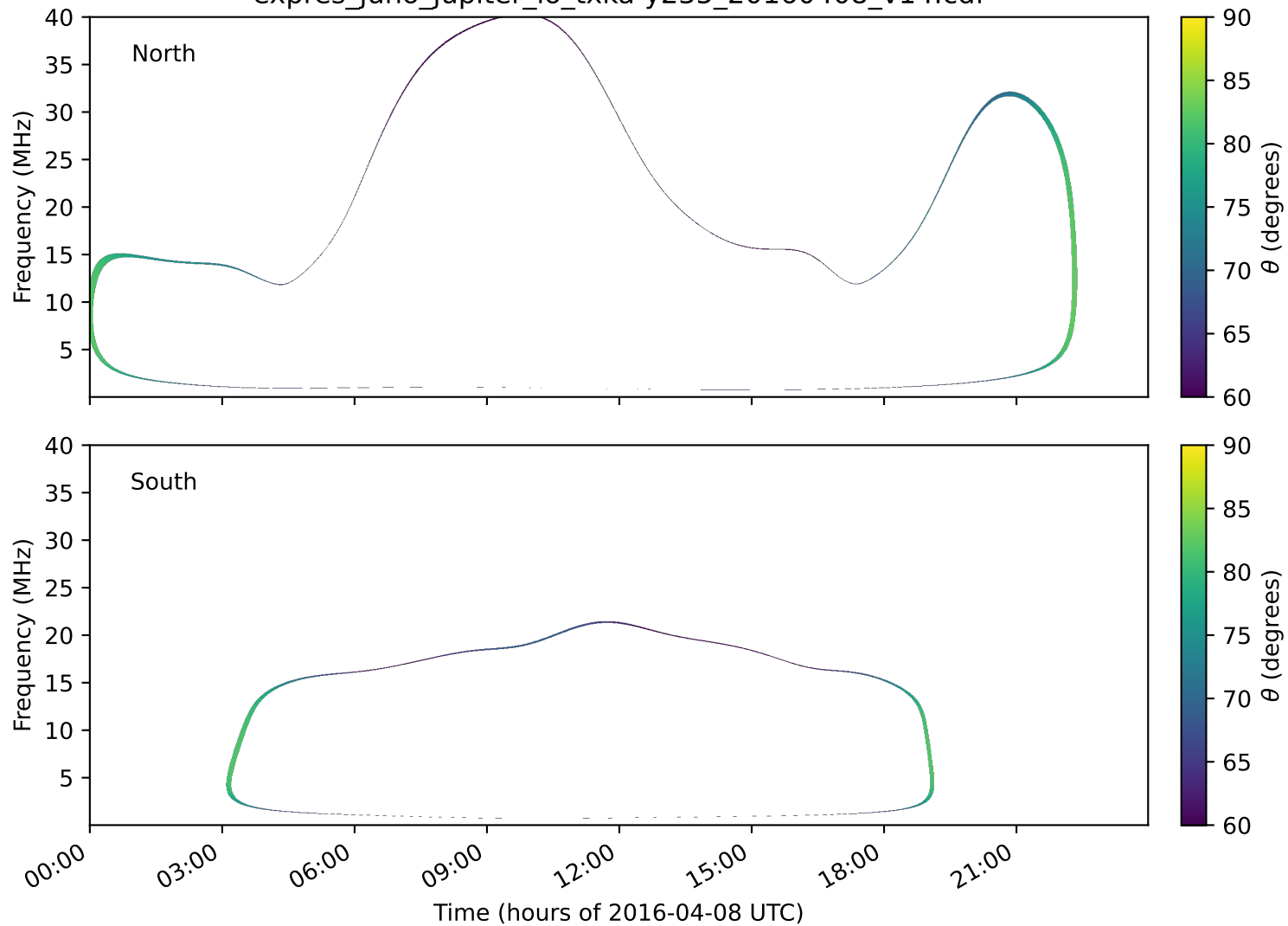
expres_juno_jupiter_io_txka-y235_20160408_v14.cdf
