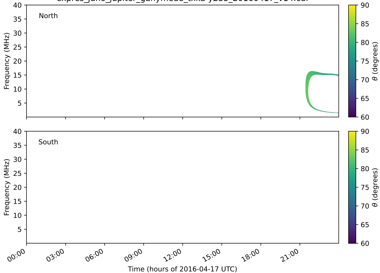
expres_juno_jupiter_ganymede_txka-y235_20160417_v14.cdf
