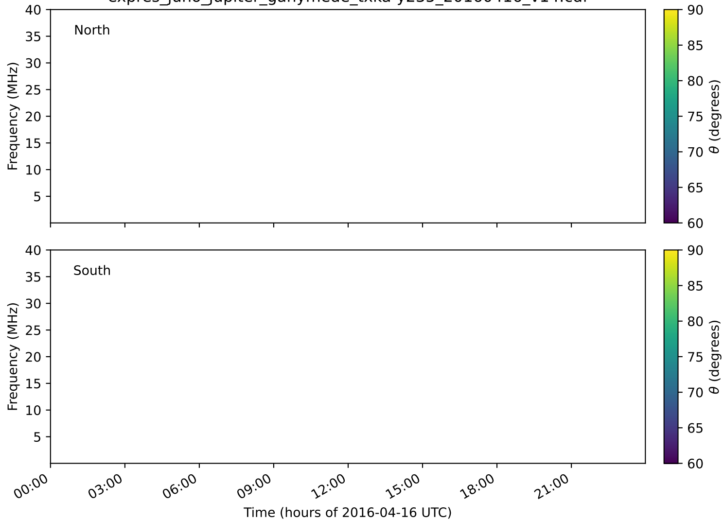
expres_juno_jupiter_ganymede_txka-y235_20160416_v14.cdf
