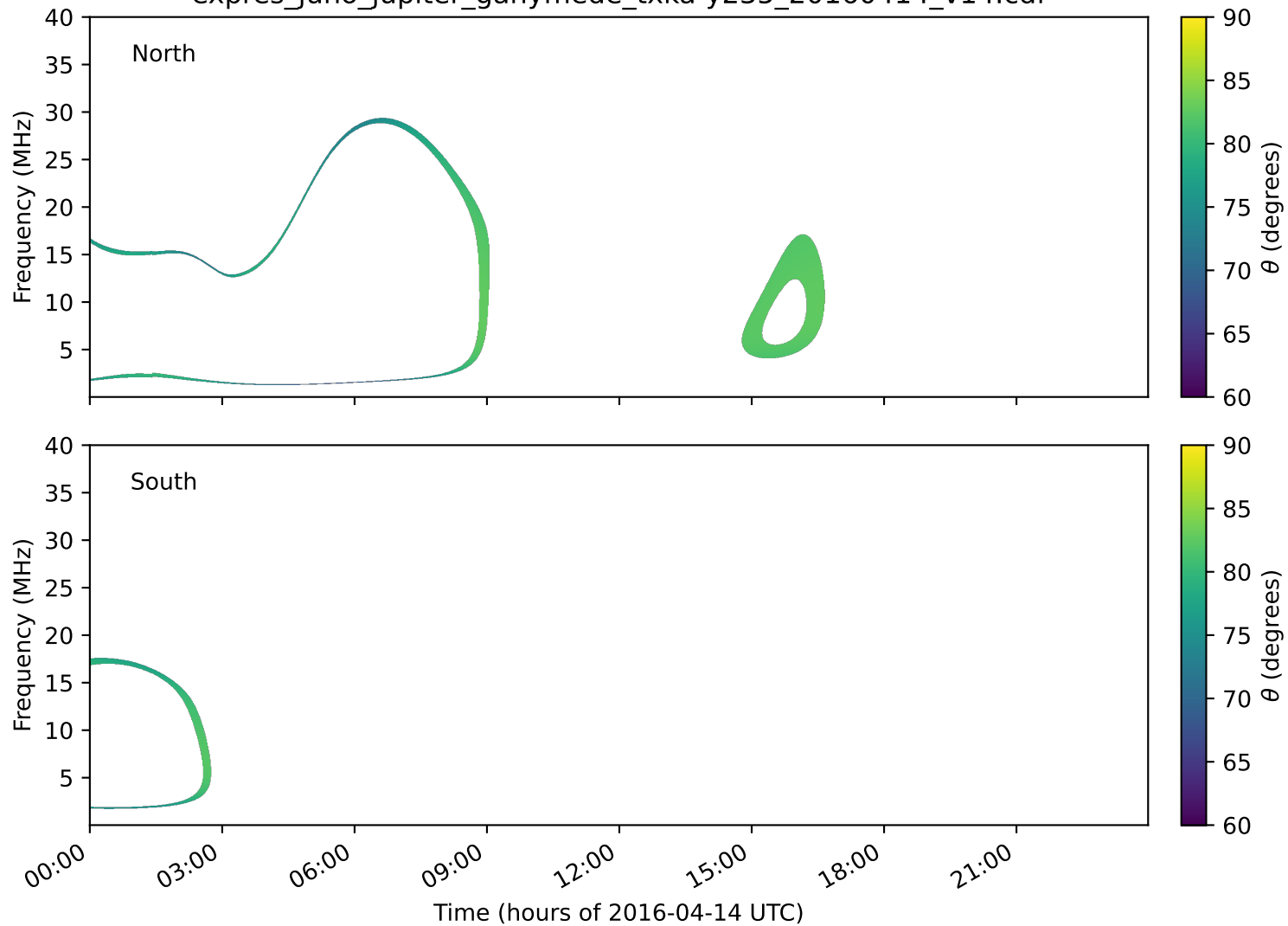
expres_juno_jupiter_ganymede_txka-y235_20160414_v14.cdf
