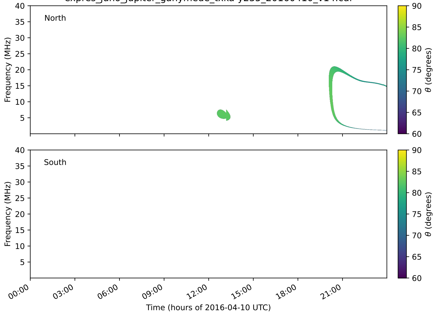
expres_juno_jupiter_ganymede_txka-y235_20160410_v14.cdf
