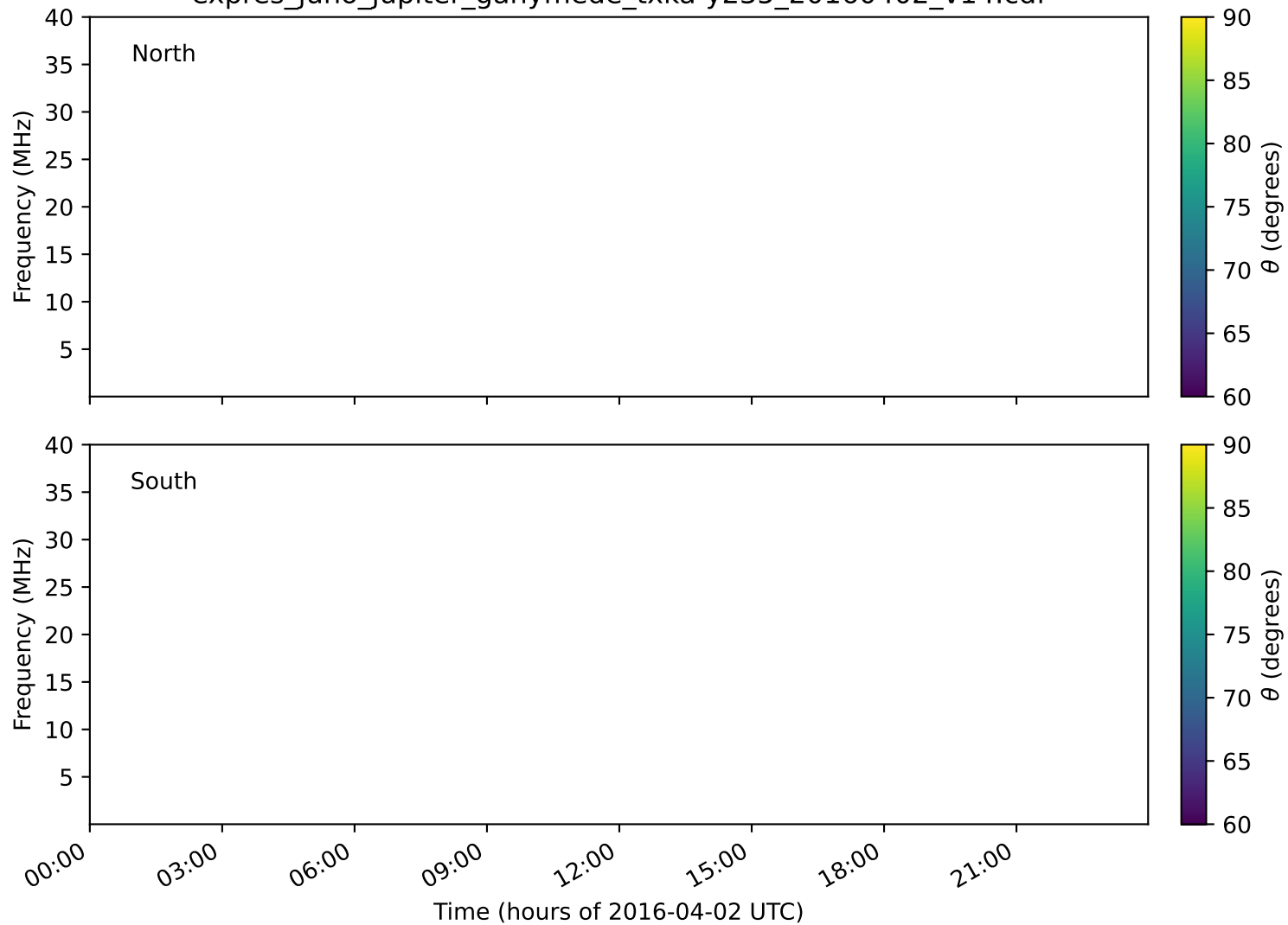
expres_juno_jupiter_ganymede_txka-y235_20160402_v14.cdf
