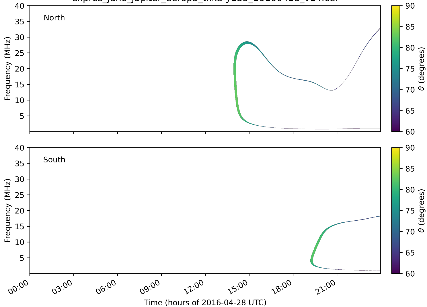
expres_juno_jupiter_europa_txka-y235_20160428_v14.cdf
