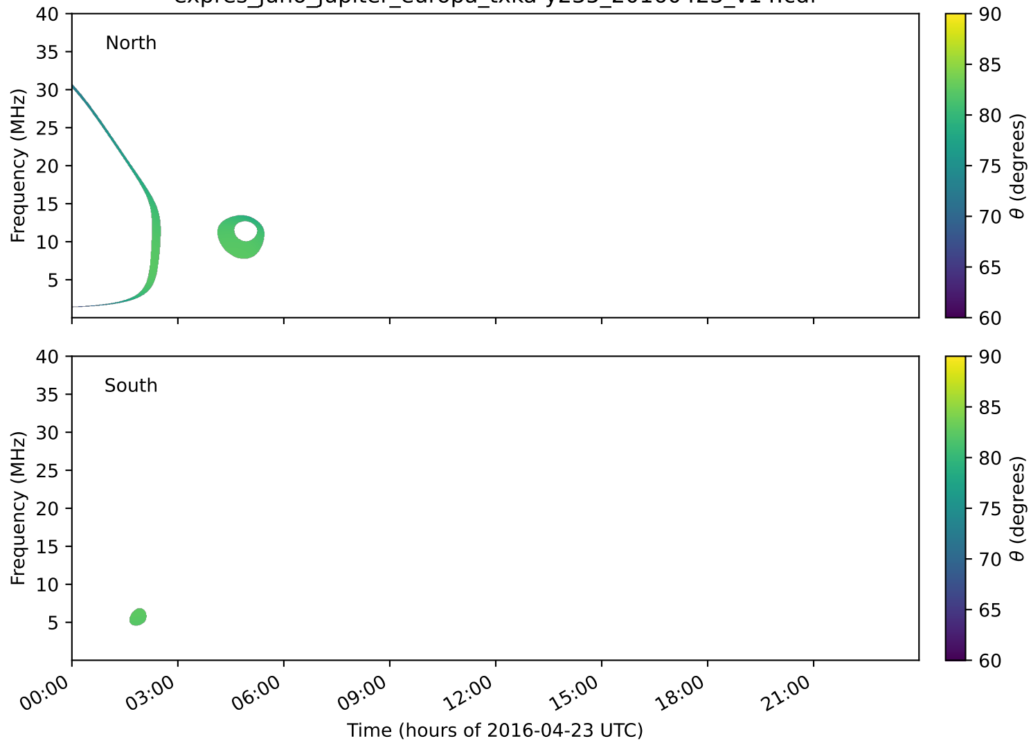
expres_juno_jupiter_europa_txka-y235_20160423_v14.cdf
