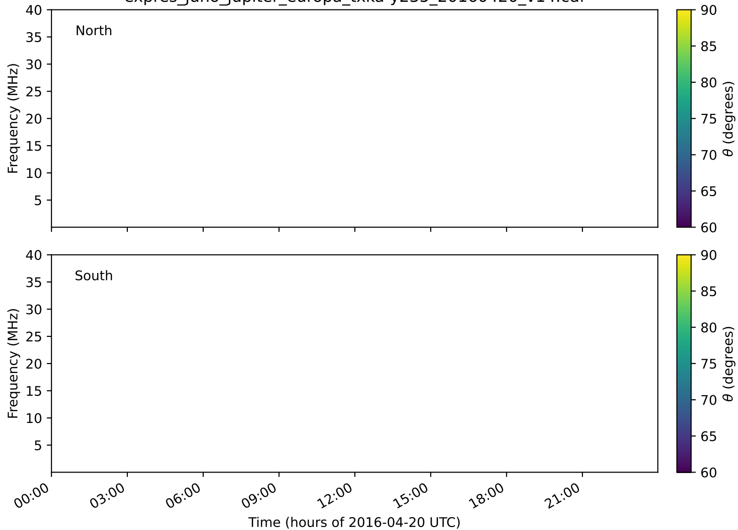
expres_juno_jupiter_europa_txka-y235_20160420_v14.cdf
