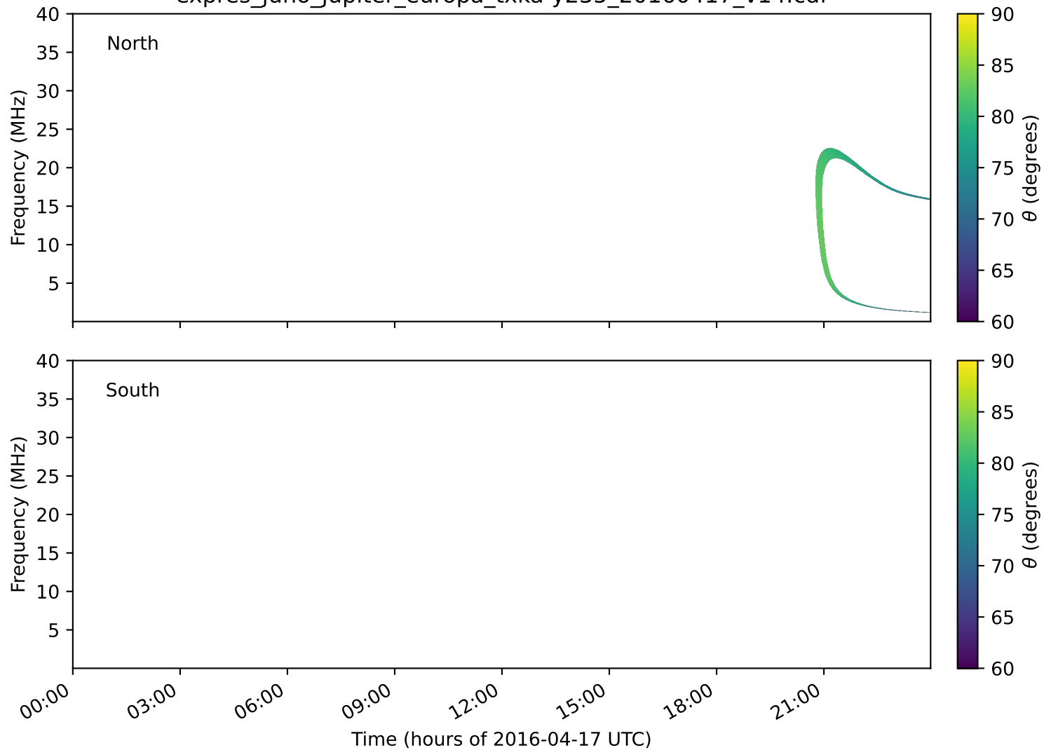
expres_juno_jupiter_europa_txka-y235_20160417_v14.cdf
