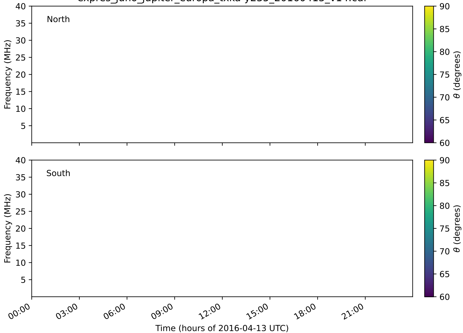
expres_juno_jupiter_europa_txka-y235_20160413_v14.cdf
