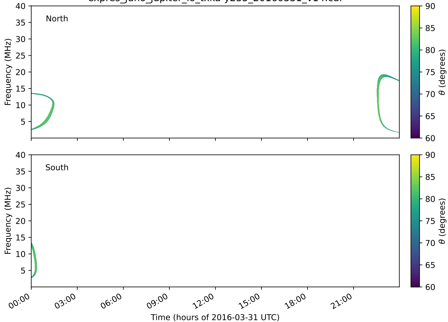
expres_juno_jupiter_io_txka-y235_20160331_v14.cdf
