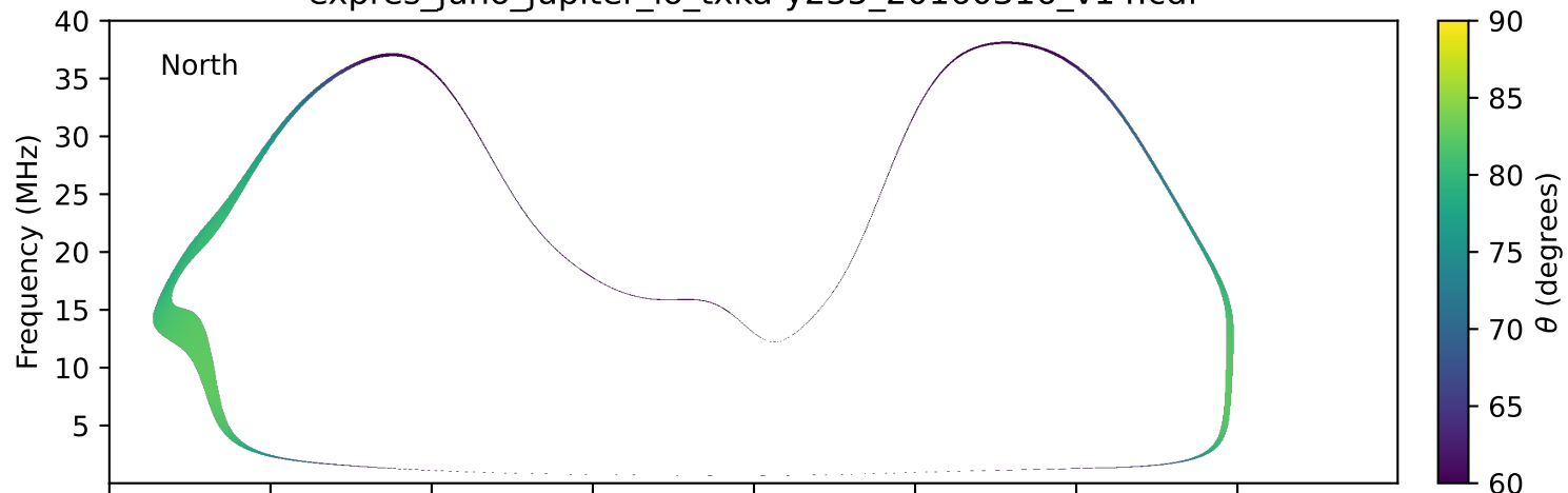
expres_juno_jupiter_io_txka-y235_20160316_v14.cdf
