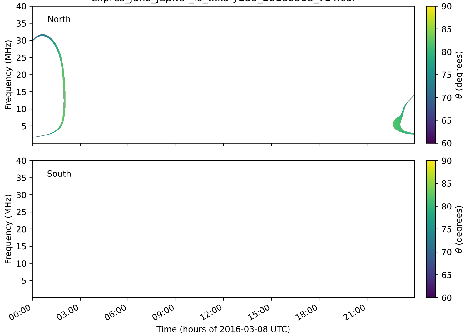
expres_juno_jupiter_io_txka-y235_20160308_v14.cdf
