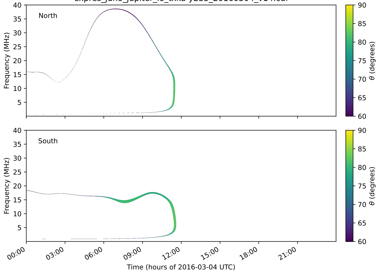
expres_juno_jupiter_io_txka-y235_20160304_v14.cdf
