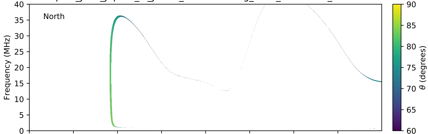
expres_juno_jupiter_io_jrm09_lossc-wid1deg_3kev_20160330_v01.cdf
