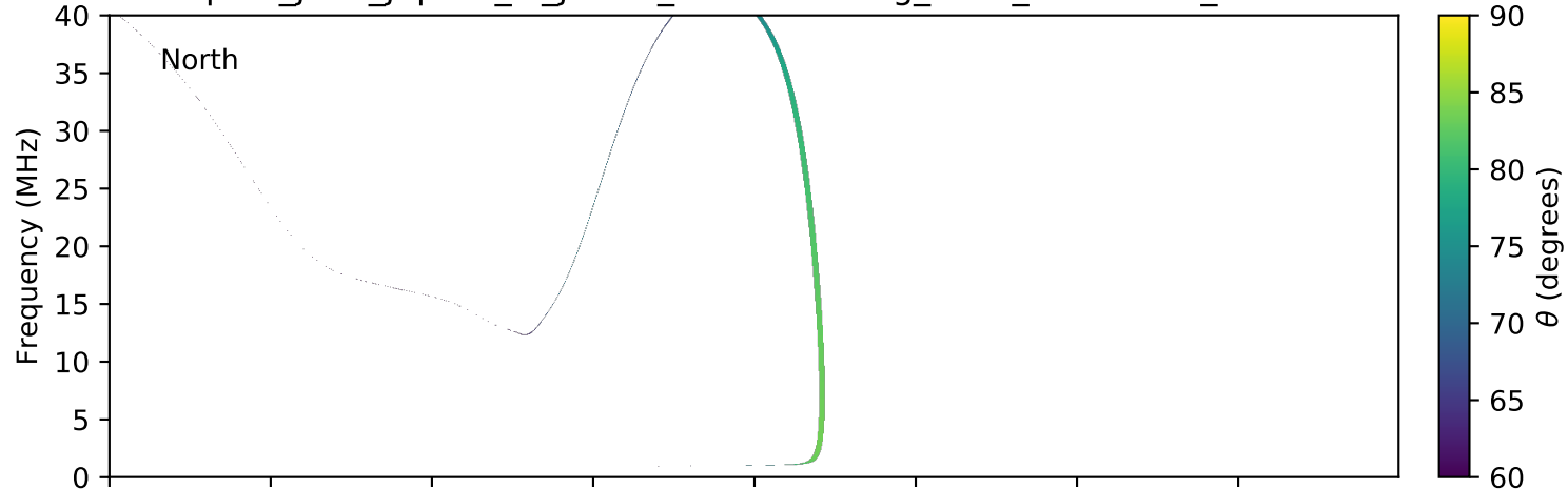
expres_juno_jupiter_io_jrm09_lossc-wid1deg_3kev_20160327_v01.cdf
