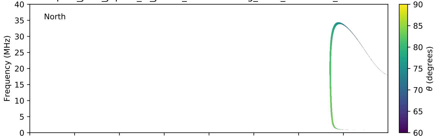
expres_juno_jupiter_io_jrm09_lossc-wid1deg_3kev_20160317_v01.cdf
