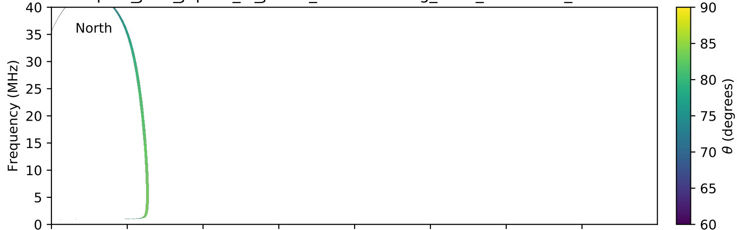
expres_juno_jupiter_io_jrm09_lossc-wid1deg_3kev_20160315_v01.cdf
