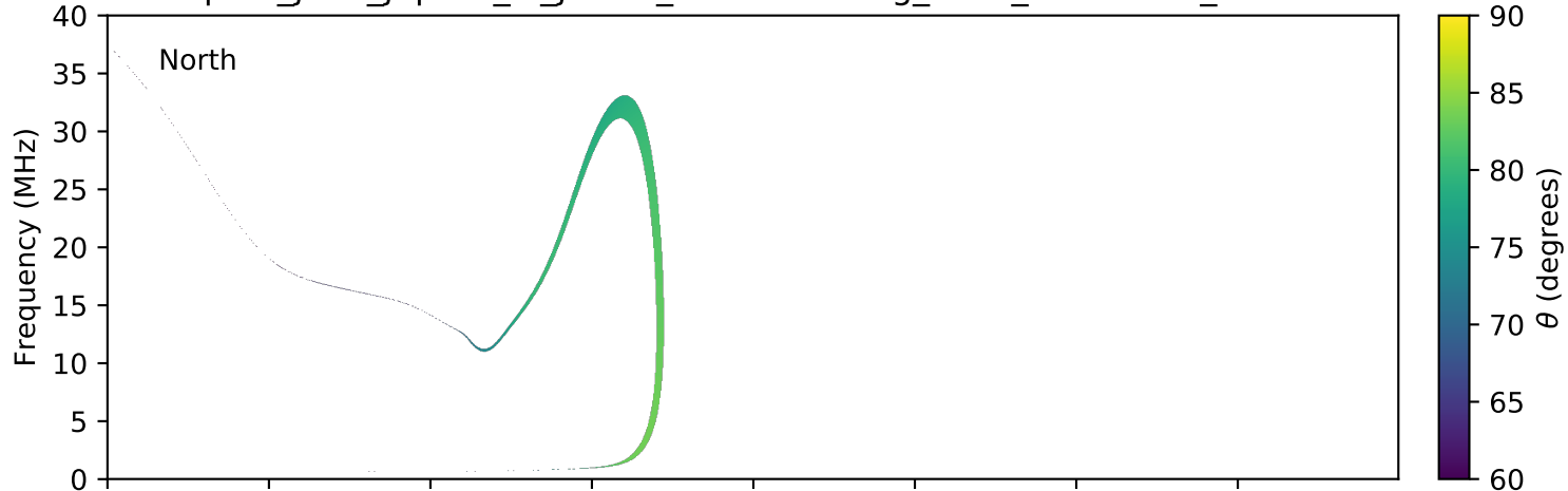
expres_juno_jupiter_io_jrm09_lossc-wid1deg_3kev_20160313_v01.cdf
