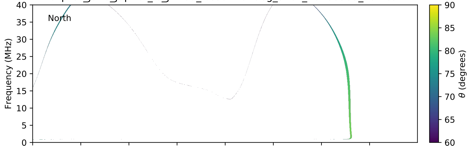
expres_juno_jupiter_io_jrm09_lossc-wid1deg_3kev_20160309_v01.cdf
