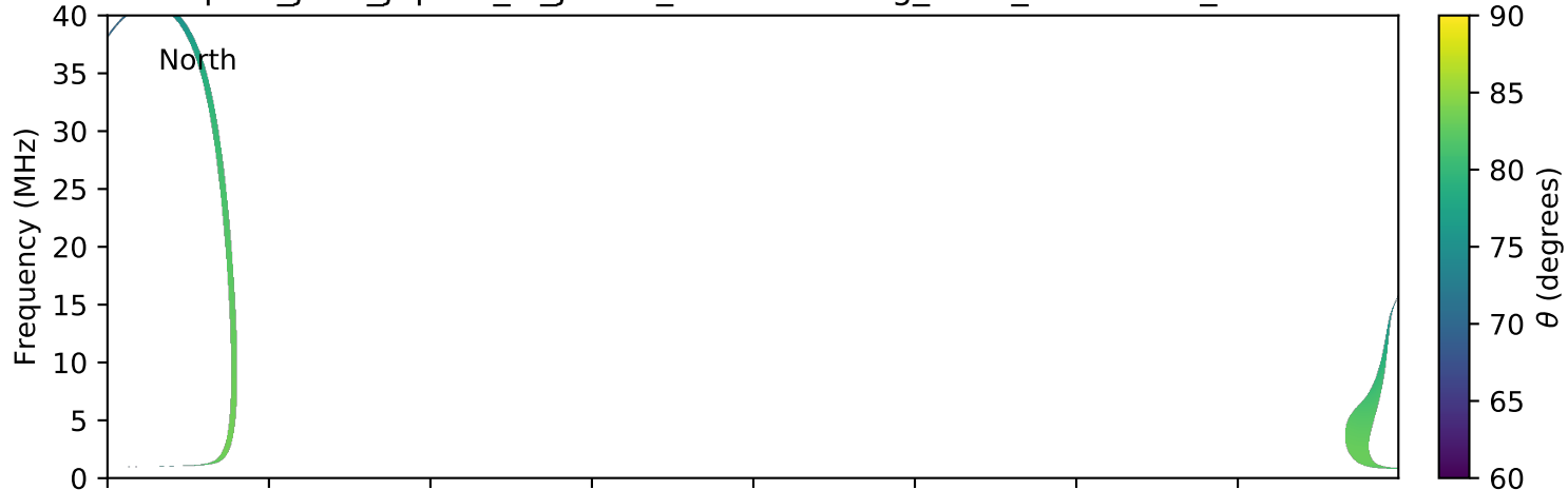
expres_juno_jupiter_io_jrm09_lossc-wid1deg_3kev_20160308_v01.cdf
