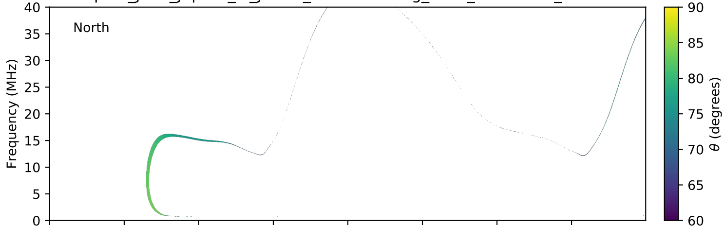
expres_juno_jupiter_io_jrm09_lossc-wid1deg_3kev_20160307_v01.cdf
