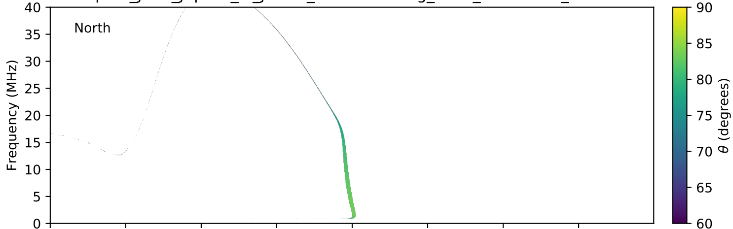
expres_juno_jupiter_io_jrm09_lossc-wid1deg_3kev_20160304_v01.cdf
