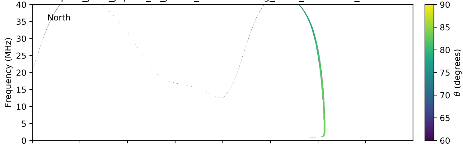
expres_juno_jupiter_io_jrm09_lossc-wid1deg_3kev_20160302_v01.cdf
