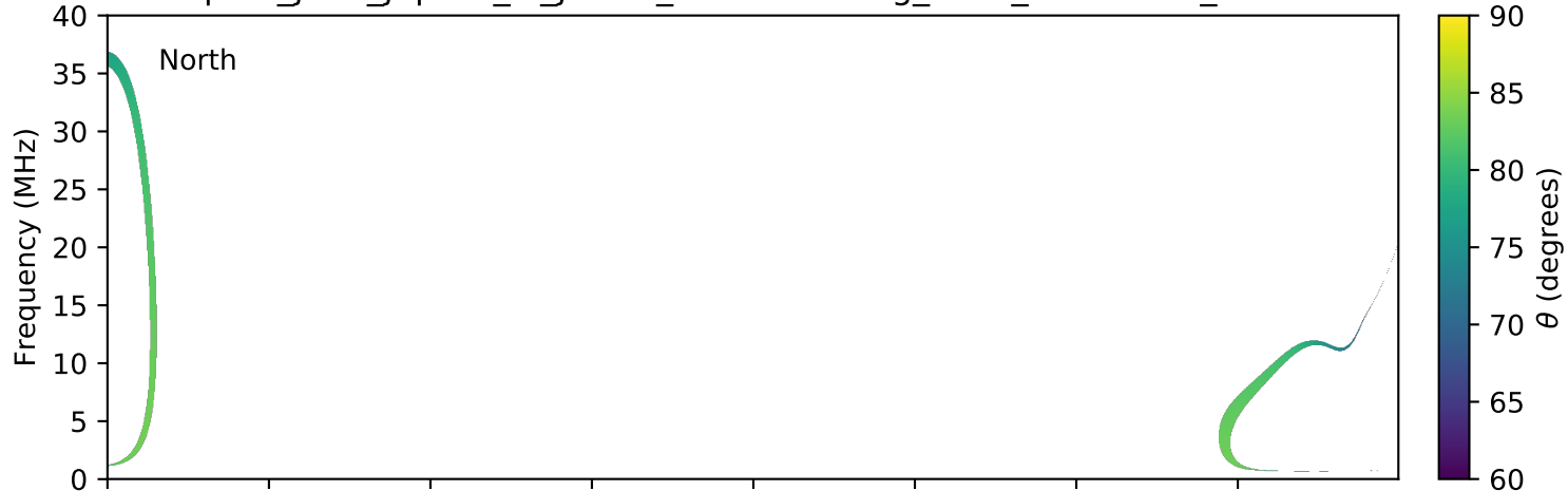
expres_juno_jupiter_io_jrm09_lossc-wid1deg_3kev_20160301_v01.cdf
