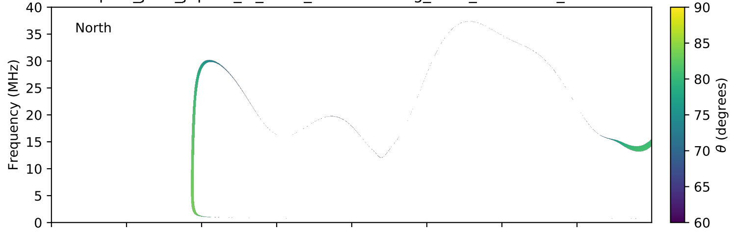
expres_juno_jupiter_io_isaac_lossc-wid1deg_3kev_20160330_v01.cdf
