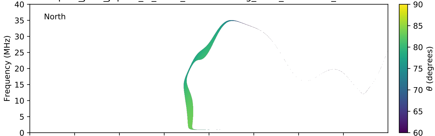
expres_juno_jupiter_io_isaac_lossc-wid1deg_3kev_20160328_v01.cdf
