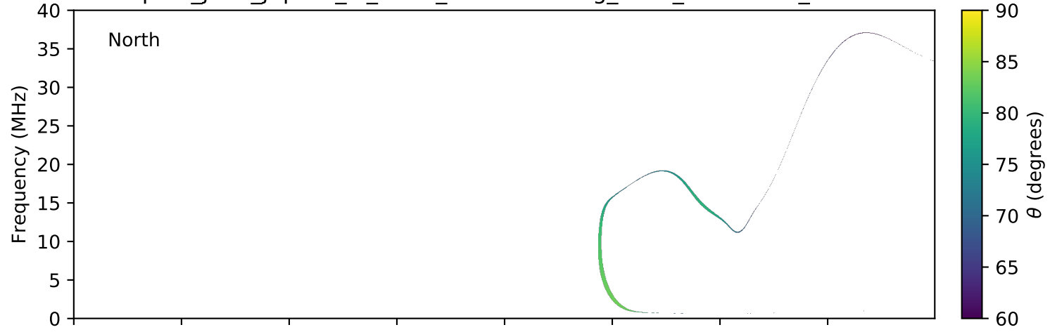
expres_juno_jupiter_io_isaac_lossc-wid1deg_3kev_20160326_v01.cdf
