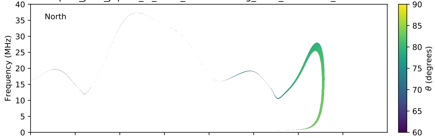
expres_juno_jupiter_io_isaac_lossc-wid1deg_3kev_20160325_v01.cdf
