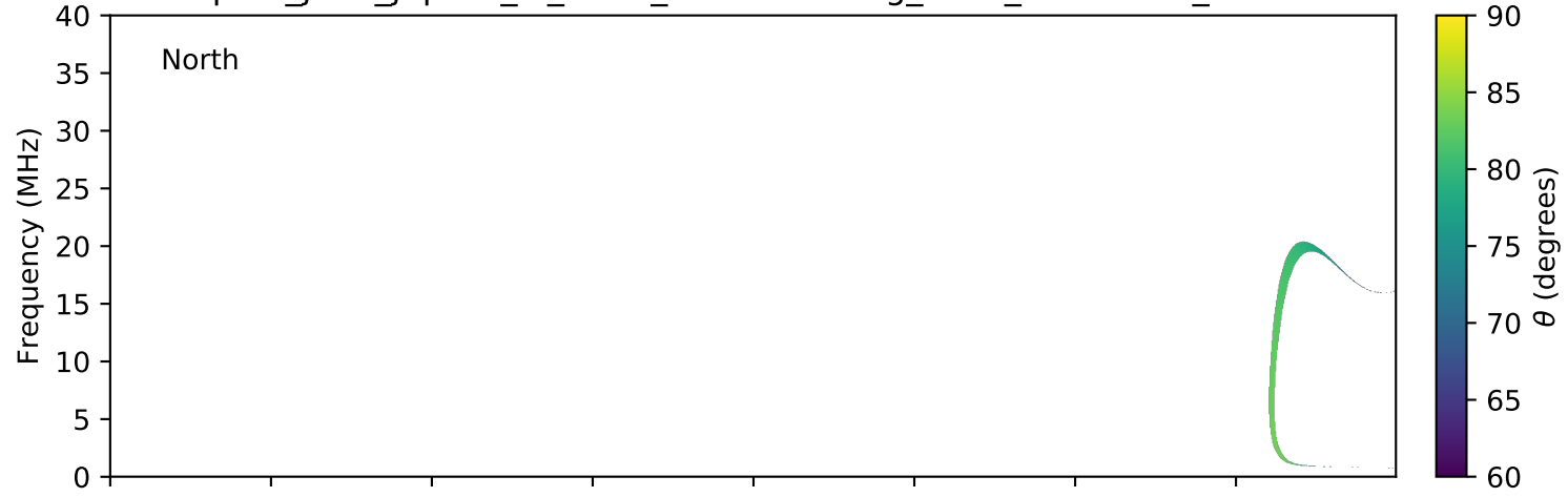
expres_juno_jupiter_io_isaac_lossc-wid1deg_3kev_20160324_v01.cdf
