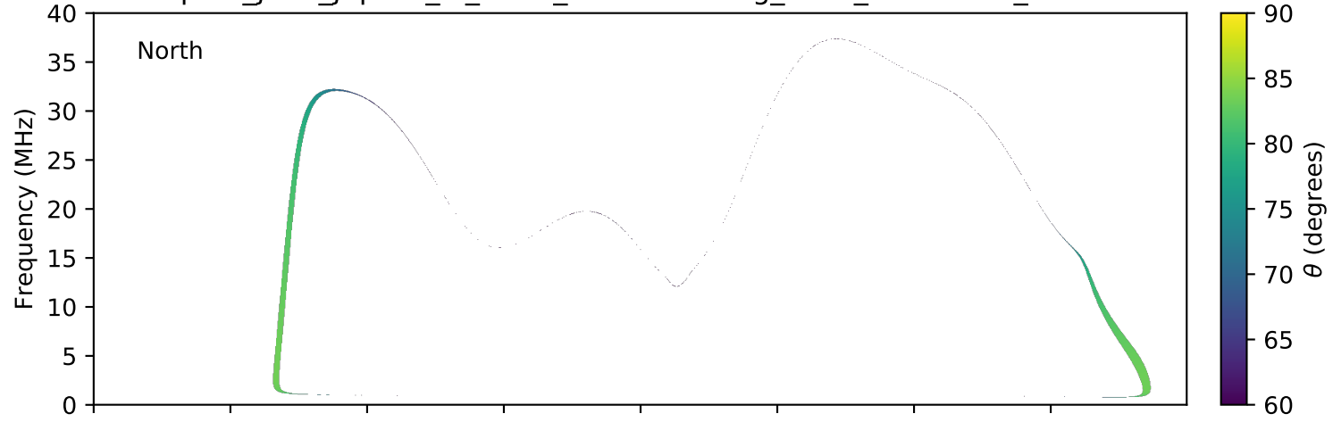
expres_juno_jupiter_io_isaac_lossc-wid1deg_3kev_20160323_v01.cdf
