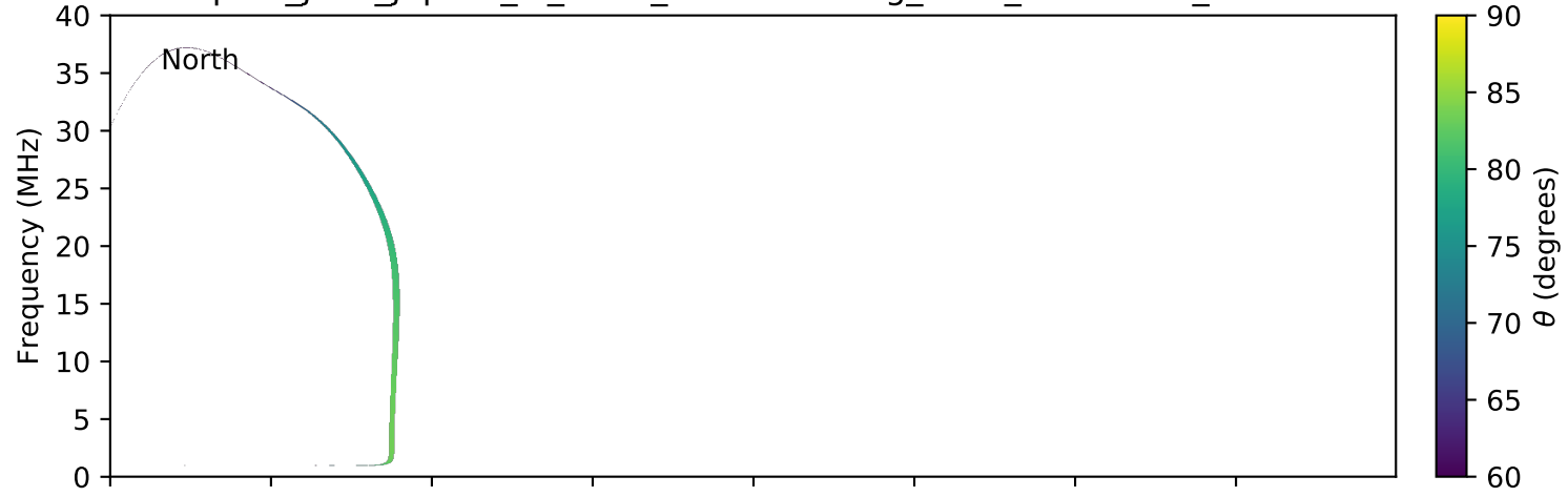
expres_juno_jupiter_io_isaac_lossc-wid1deg_3kev_20160322_v01.cdf
