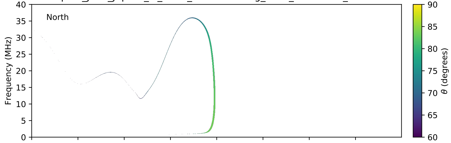
expres_juno_jupiter_io_isaac_lossc-wid1deg_3kev_20160320_v01.cdf
