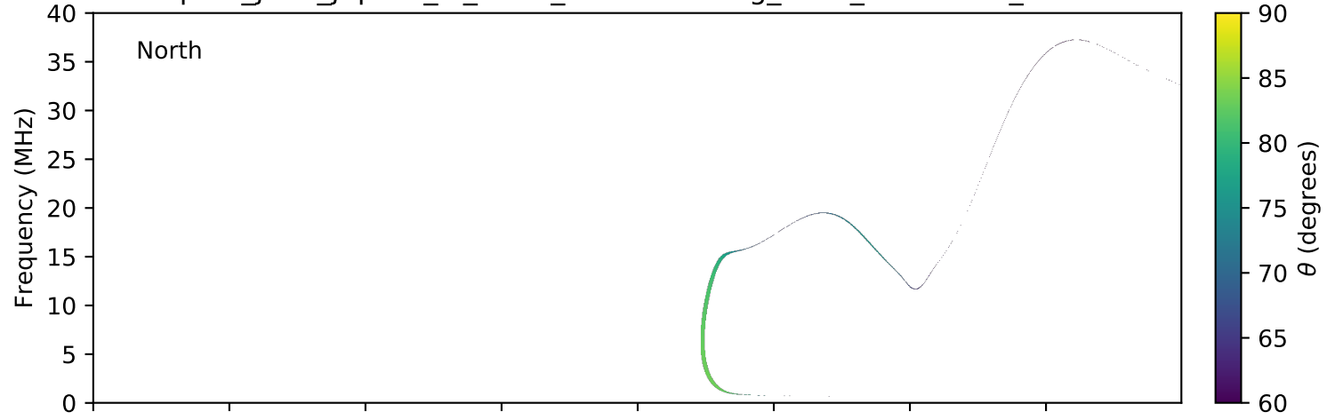
expres_juno_jupiter_io_isaac_lossc-wid1deg_3kev_20160319_v01.cdf
