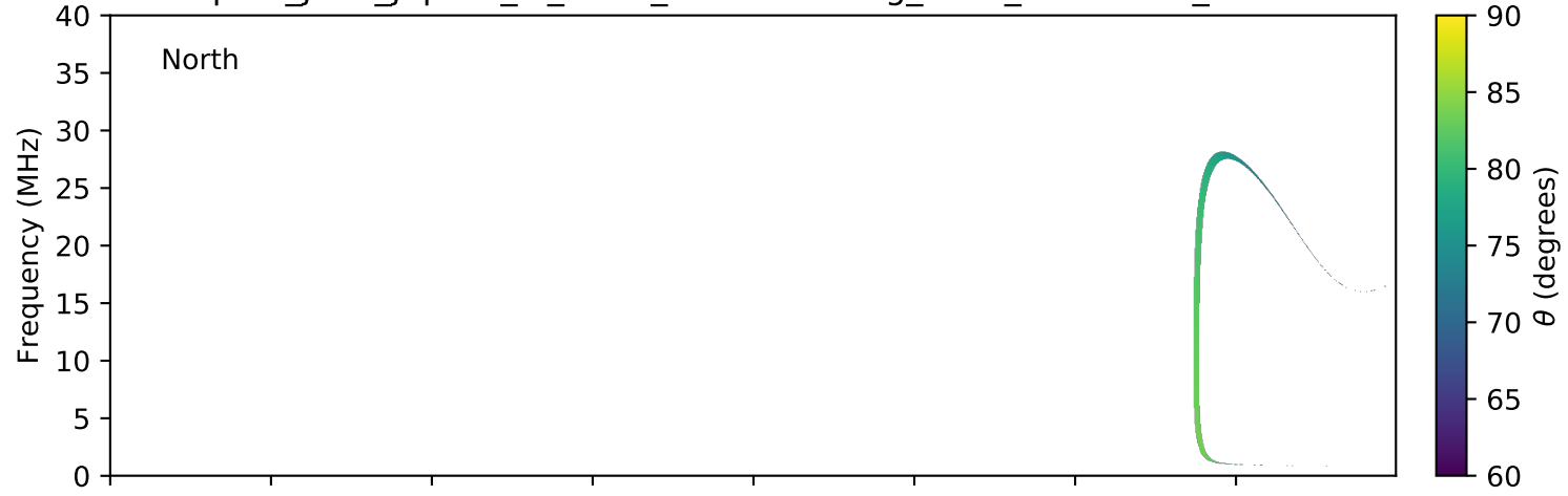
expres_juno_jupiter_io_isaac_lossc-wid1deg_3kev_20160317_v01.cdf
