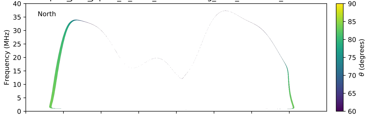
expres_juno_jupiter_io_isaac_lossc-wid1deg_3kev_20160316_v01.cdf
