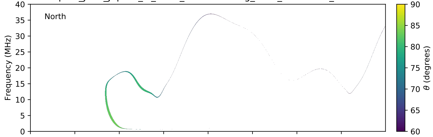
expres_juno_jupiter_io_isaac_lossc-wid1deg_3kev_20160314_v01.cdf
