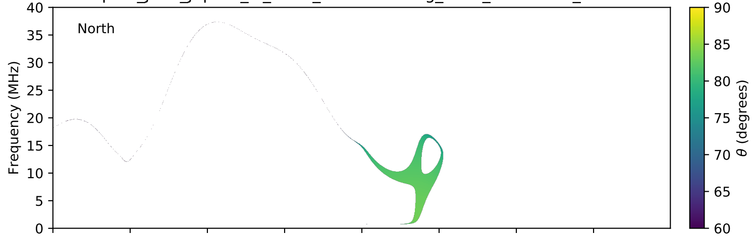
expres_juno_jupiter_io_isaac_lossc-wid1deg_3kev_20160311_v01.cdf
