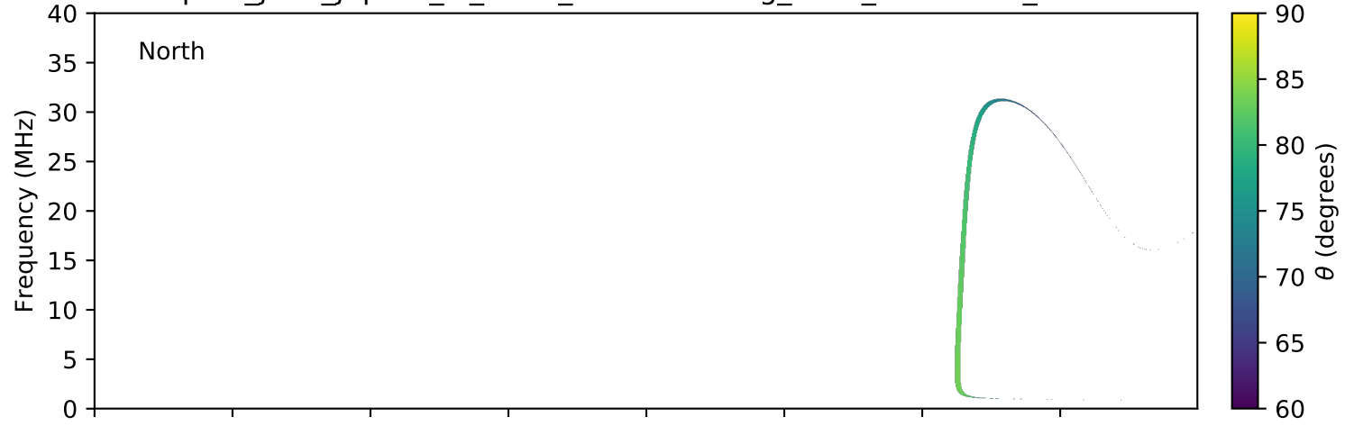
expres_juno_jupiter_io_isaac_lossc-wid1deg_3kev_20160310_v01.cdf
