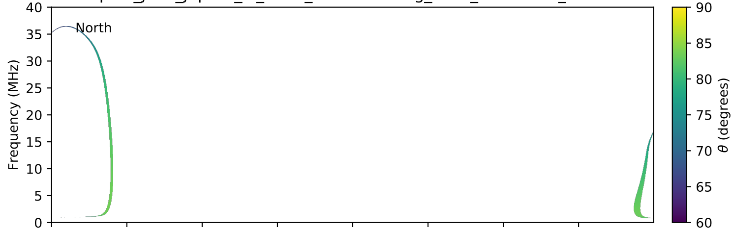
expres_juno_jupiter_io_isaac_lossc-wid1deg_3kev_20160308_v01.cdf
