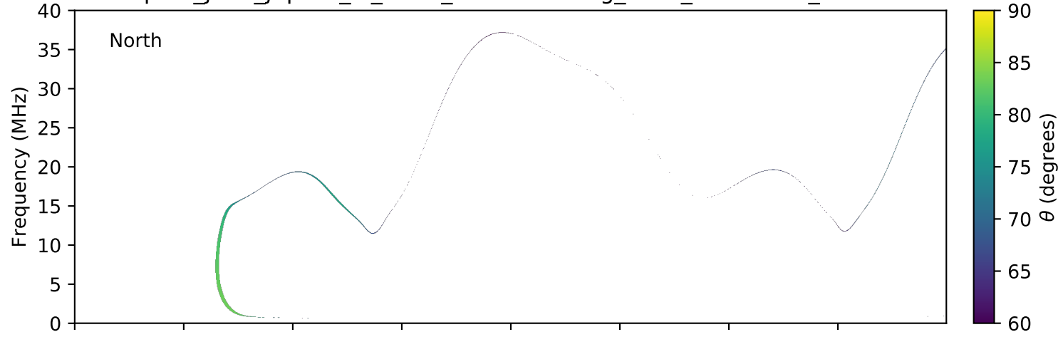
expres_juno_jupiter_io_isaac_lossc-wid1deg_3kev_20160307_v01.cdf
