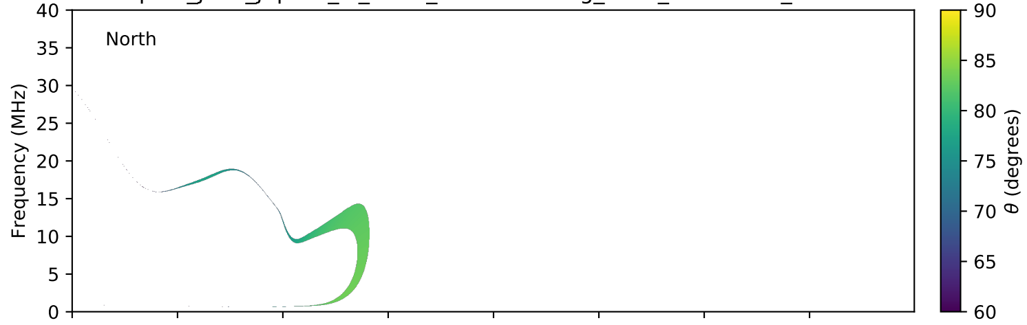
expres_juno_jupiter_io_isaac_lossc-wid1deg_3kev_20160306_v01.cdf
